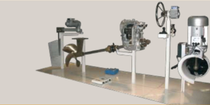
Shaftline System
