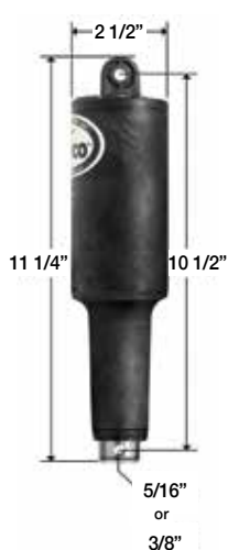
101 XD Actuator 2 1/4" Stroke (5.715 cm)
