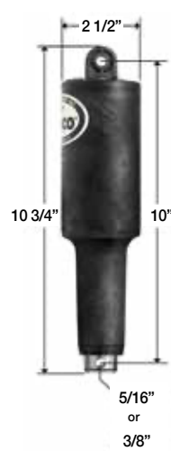
101 XDS (Short) Actuator 2 1/4" Stroke (5.715 cm)
