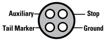
TRAILER END
